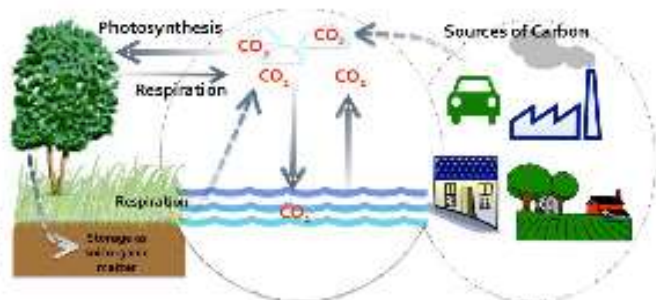
The Carbon Cycle
